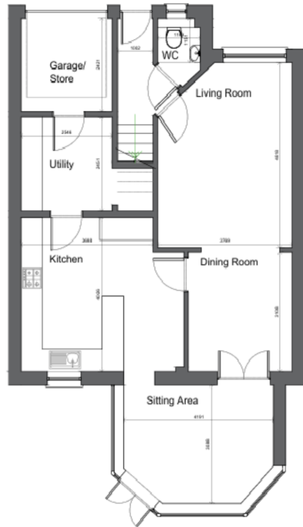
Floor Plan as Existing 1:50 1m 0 1m 2m 3m
