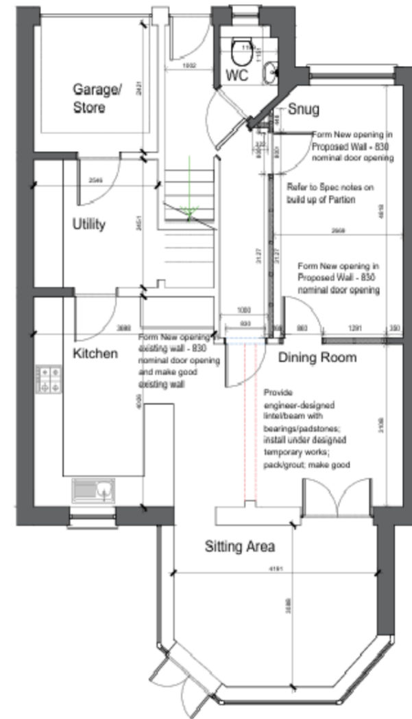
Floor Plan as Proposed 1:50 1m 0 1m 2m 3m
